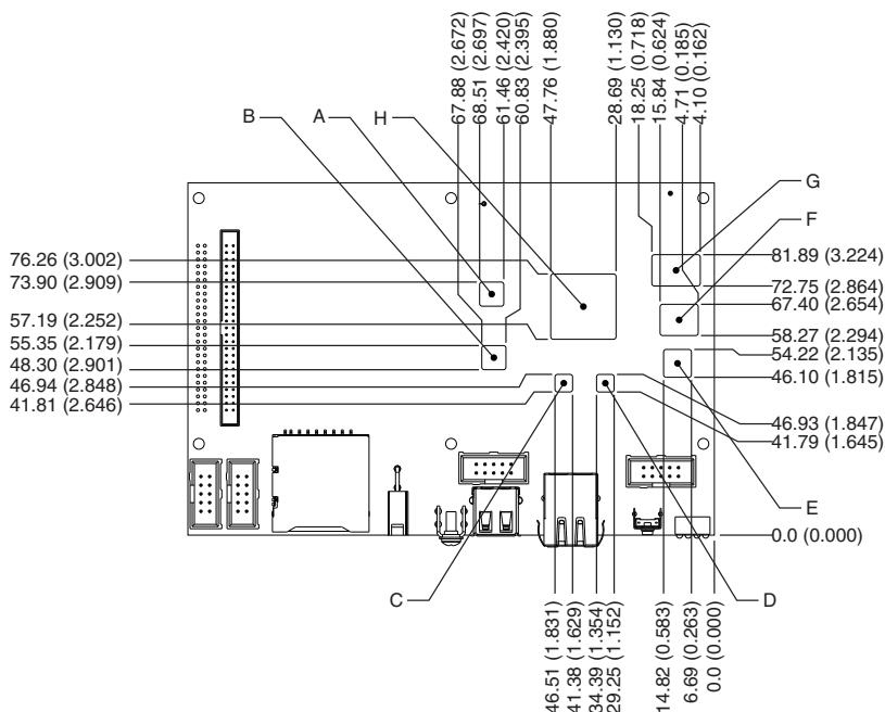
Figure 13. sbRIO-9627 Pedestal Dimensions in mm (in.)
